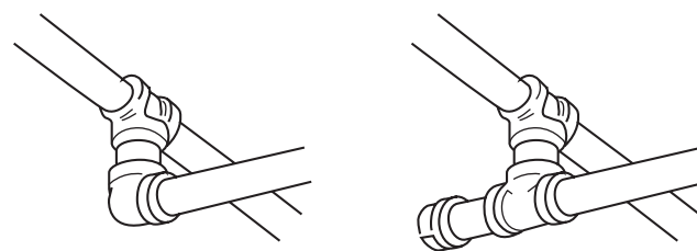
FIGURE D.3.2(a) Replacement of Elbow at End of Cross Main with Flushing Connection Consisting of 50 mm (2 in.) Nipple and Cap.
